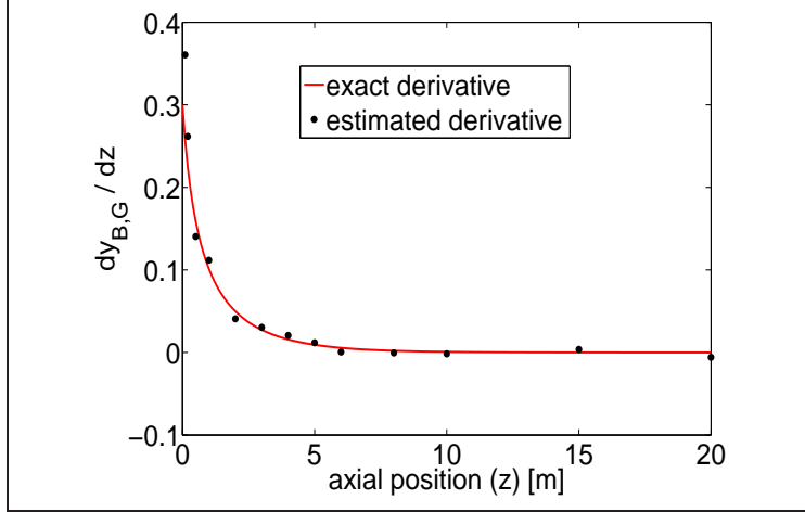
Figure 2: Estimated and exact derivative.
