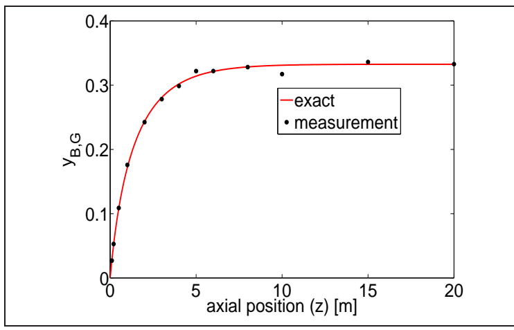
Figure 1: Measurements and exact trajectory.
