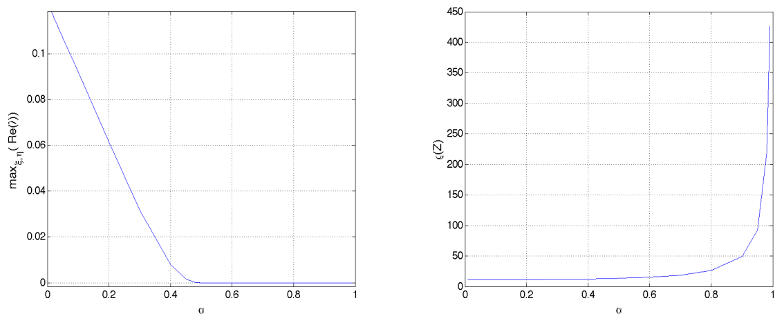
(a) \max_{\xi, \eta} \operatorname{Re}(\lambda(\xi, \eta)) as a function of the scaling parameter \alpha . (b) \max_{\xi, \eta} \rho(Z(\xi, \eta)) as a function of the scaling parameter \alpha .
